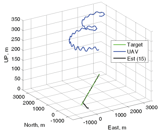
Fig. 10 2-D and 3-D projections of relative motion.
